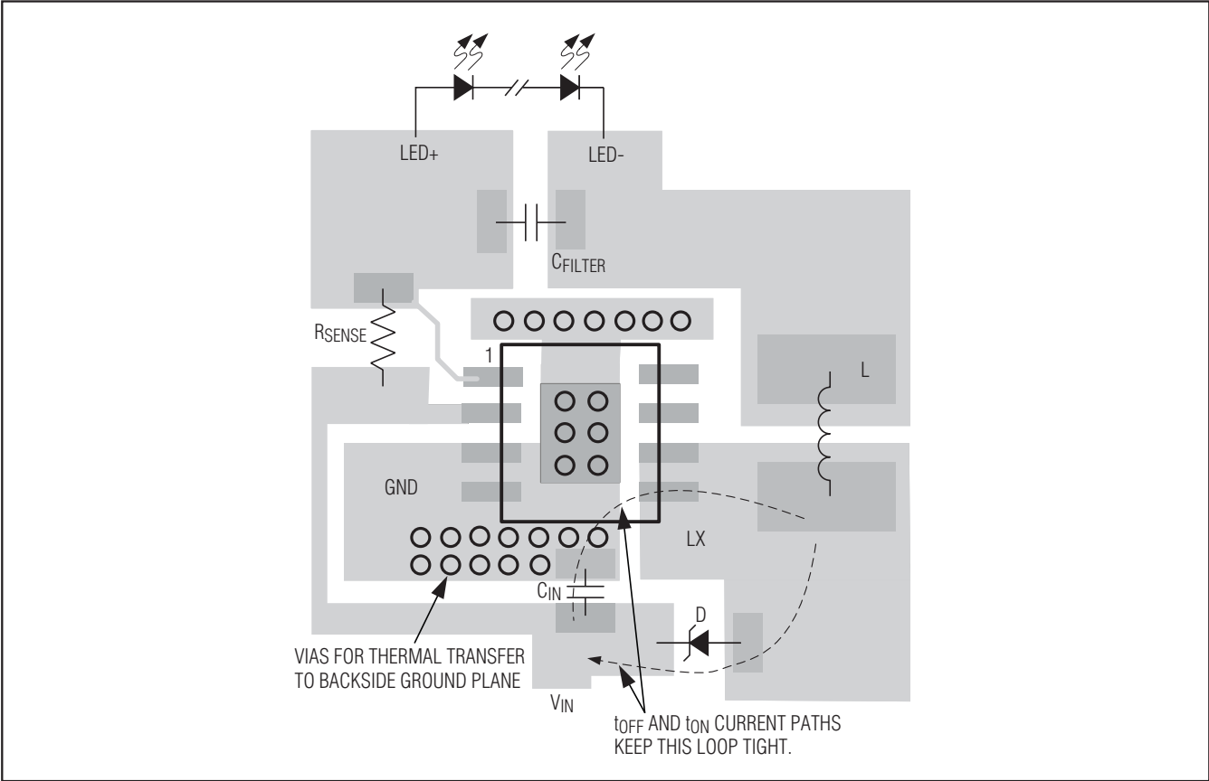
Figure 3. PCB Layout
