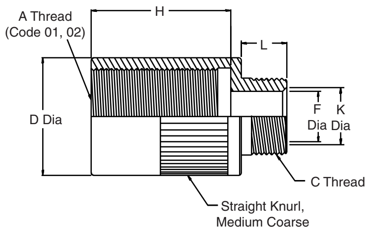
STYLE 01 ADAPTER WITH INTERNAL "A" THREAD
